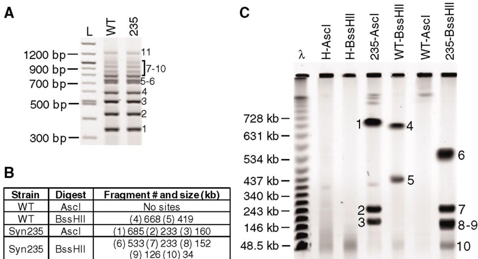
Fig. 3. Characterization of the synthetic genome isolated from yeast. (a) Yeast clones containing a completely assembled synthetic genome were screened by multiplex PCR with a primer set that produces 11 amplicons; one at each of the 11 assembly junctions. Yeast clone sMmYCp235 (235) produced the 11 PCR products expected for a complete genome assembly. For comparison, the natural genome extracted from yeast (WT) was also analyzed. PCR products were separated on a 2% E-gel (Invitrogen). L indicates the 100-bp ladder (NEB). (b) The sizes of the expected Asc I and BssH II restriction fragments for natural (WT) and synthetic (Syn235) M. mycoides genomes. (c) Natural (WT) and synthetic (235) M. mycoides genomes were isolated from yeast in agarose plugs. In addition, DNA was purified from the host strain alone (H). Agarose plugs were digested with Asc I or BssH II and fragments were separated by clamped homogeneous electrical field (CHEF) gel electrophoresis. Restriction fragments corresponding to the correct sizes are indicated by the fragment numbers shown in (b).
